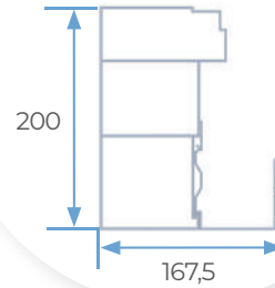
3 | STD BEAM
