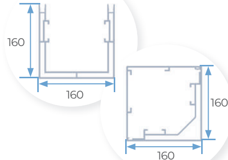
5B | CLOSED PILLAR
